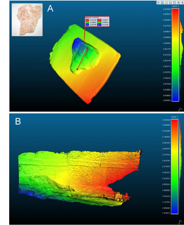
Fig. 16. 3D mapping. (a) Close range 3D mapping image done in the Boulby Mine with a rock sample. (b) Long range 3D mapping of the wall of the mine shaft. The small box on the bottom right of the image is the PACKMAN instrument.
