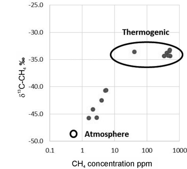
Fig. 14. Methane concentrations, sampled in the atmosphere within 13 locations in the Boulby Mine tunnels, plotted against their respective δ 13 C-CH 4 values. The simplest explanation for the range of values is mixing between a thermogenic source and an atmospheric (ambient surface derived air) source. The value for the atmosphere endmember is taken from Whiticar (1999).
